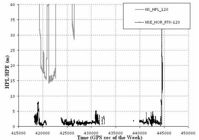
Figure 5: Route A EGNOS Operational HPE/HPL time series.
