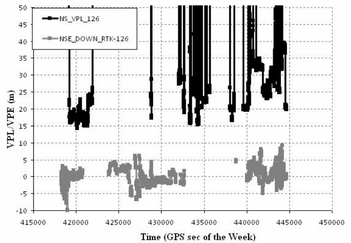
Figure 4: Route A EGNOS Test VPE/VPL time series.
