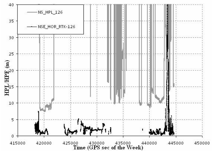
Figure 3: Route A EGNOS Test HPE/HPL time series.
