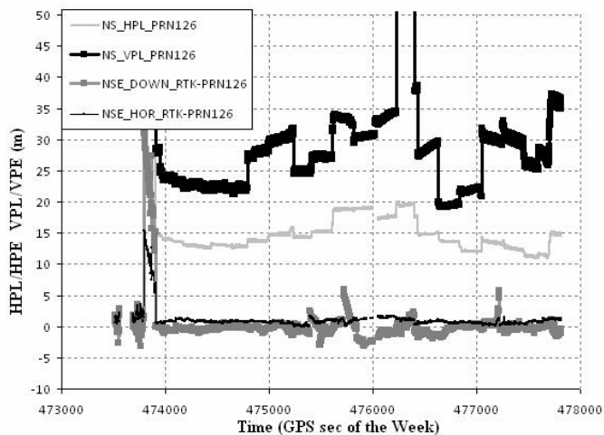
Figure 14: Route I EGNOS SiSNet Test HPE/HPL VPE/VPL time series.
