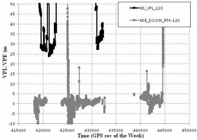
Figure 6: Route A EGNOS Test VPE/VPL time series.
